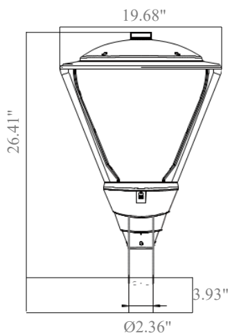
LED A
