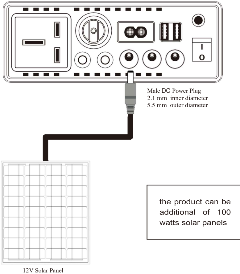
Figure 10. Adding external solar panel
