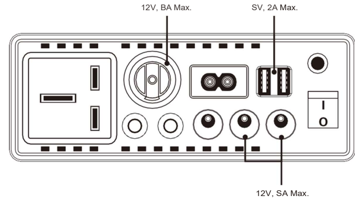
Figure 7. Maximum current ratings for DC outputs
